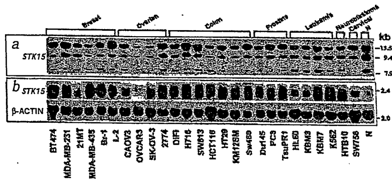
Fig. 1 Southern- and northern-blot hybridization analyses estimating STK15 copy number (a) and STK15 mRNA expression (b) in tumour cell lines. The top band of approximately 13.5 kb in the Bam HI digests, representing STK15 -specific sequences, and the third band of approximately 7.9 kb, representing unamplified sequences, were included in signal intensity measurements to estimate gene copy number. Lane N contained human lymphocyte DNA from a normal healthy individual. The names of cell lines from which DNA were derived are indicated. The highest level of amplification (8x) was seen in the breast tumour cell lines BT474 and MDA-MB-231, whereas approximately 2.5x to 5x amplification was seen in ovarian (2774), colon (DIF1, H716, KM12SM, SW480), prostate (PC3, TsuPR1), neuroblastoma (HTB10) and cervical (SW756) tumour cell lines.
